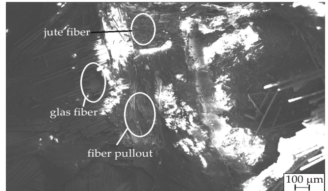
Fig. 8. SEM image of specimen D showing microcrack
