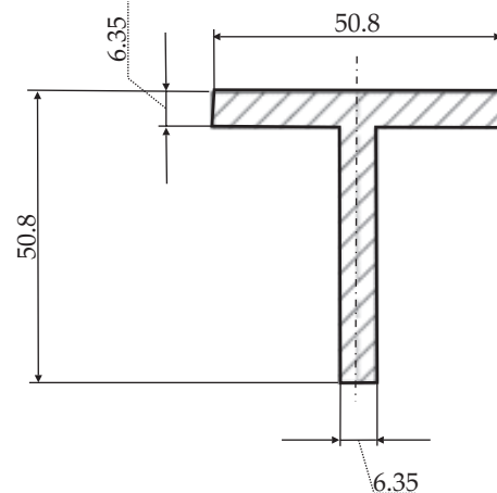
Fig. 2. Dimensions of cross-section of T-beam
