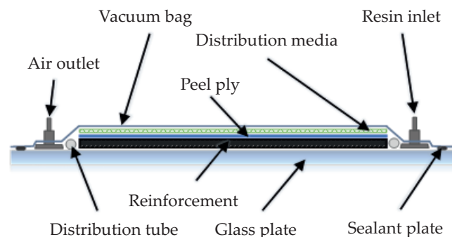
Fig. 2. Scheme of the composite manufacturing system using the infusion method
