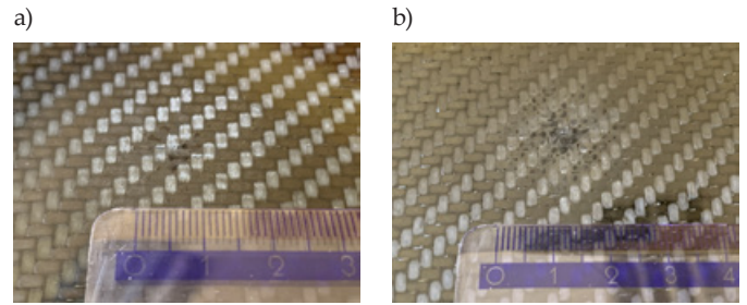
Fig. 6. Photographs of damage areas of EP_0.5%CB/CF composite: a) after one impulse, b) five impulses
