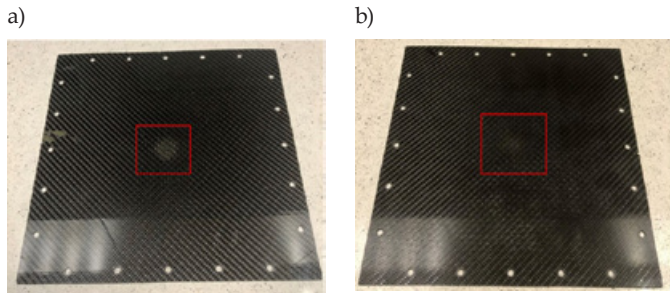
Fig. 5. Photographs of the surface after impact testing of composites: a) EP/CF, b) EP_0.5%CB/CF
