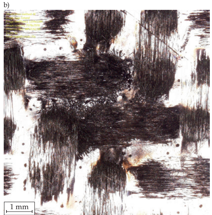
Fig. 7. Microscopic images of the damage center of EP_0.5%/CB/CF composite: a) one impulse, b) five impulses; 35× magnification
