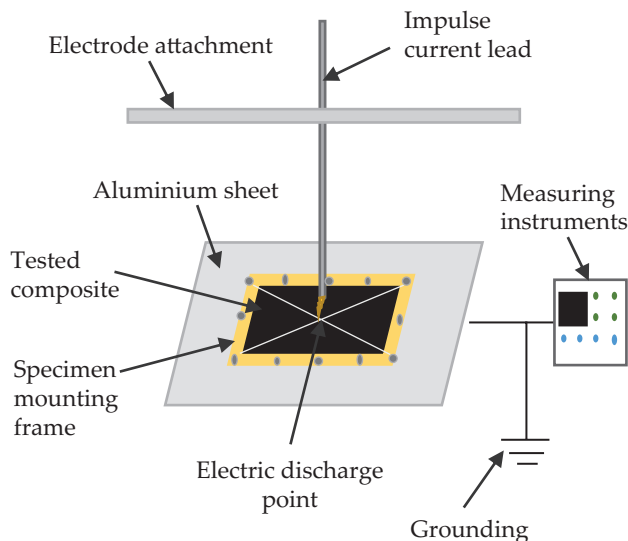
Fig. 3. System for testing the resistance of polymer composites to lightning discharges
