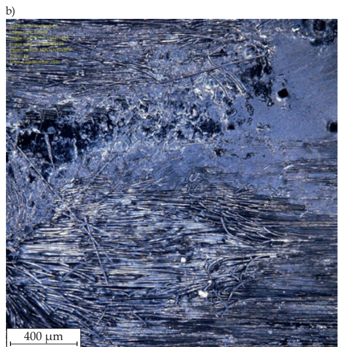
Fig. 8. Microscopic images of the damage center of EP_0.5%/CB/CF composite: a) one impulse, b) five impulses; 139× magnification
