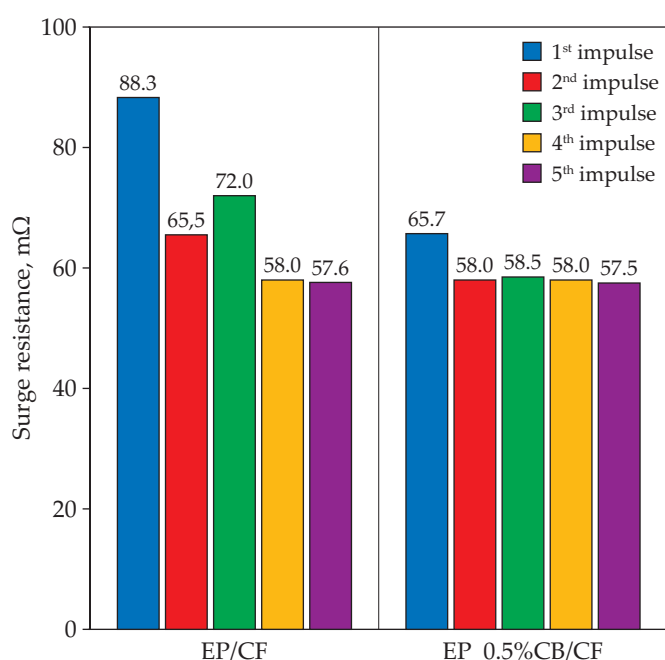
Fig. 4. Surge resistance of composites for successive current pulses
