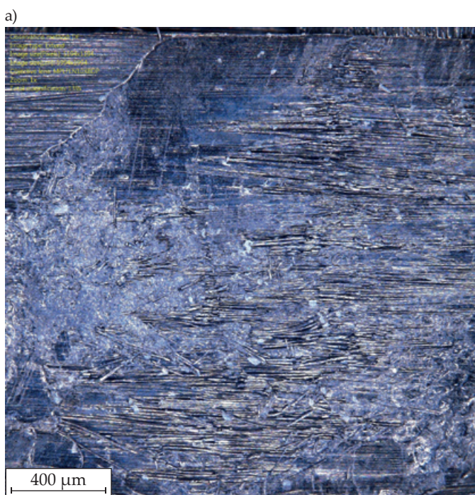
Fig. 8. Microscopic images of the damage center of EP_0.5%/CB/CF composite: a) one impulse, b) five impulses; 139× magnification
