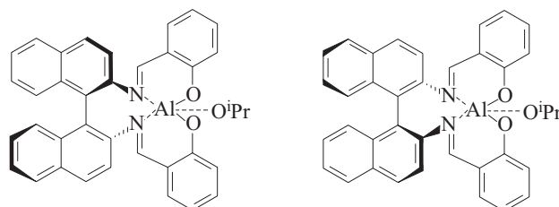
Scheme F. Structures of catalysts – >AlO^iPr with chiral ligands: ( R )-SBO 2 -AlO i Pr (left) and ( S )-SBO 2 -AlO i Pr (right)
