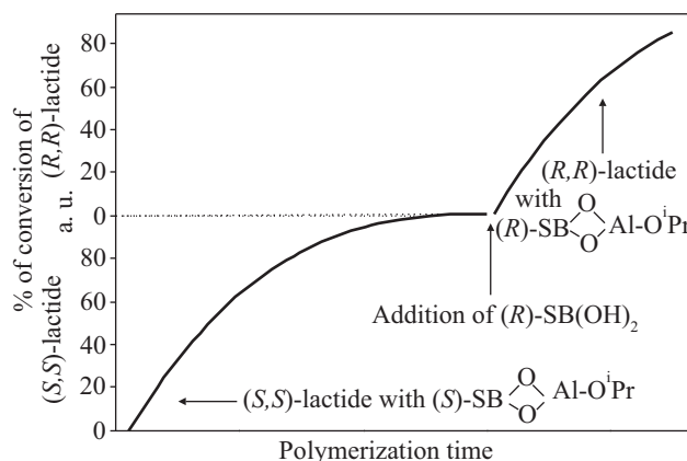
Fig. 1. Simplified kinetics of block copolymer and stereocomplex formation; stereoselective polymerization of racemic LA: first ( S,S )-LA and then ( R,R )-LA in consecutive order, governed by >AlOR catalyst, first with ( S )-ligand and then with ( R )-ligand; the detailed data (polymerization conditions) are given in the original paper [1]
